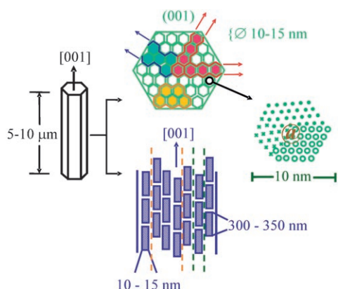
Figure 2. Diagram of the nanocomposite inner architecture of a young fluorapatite–gelatine seed derived from HRTEM investigations. [12,13]
